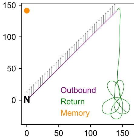
Random
