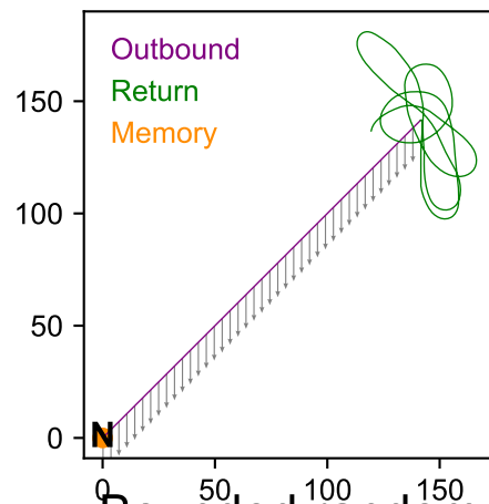
Bounded random
