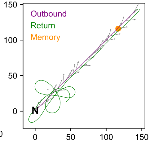
Bounded random
