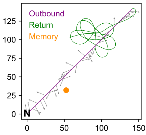
Random
